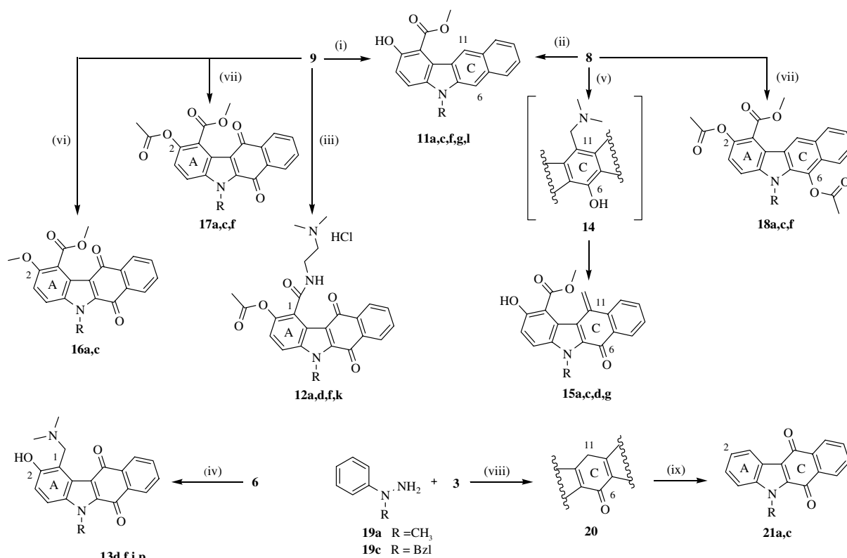
Scheme 4. Reagents and conditions: (i) 4equiv Zn/HOAc/reflux/6h; (ii) 4equiv Zn/HOAc/reflux/12h; (iii) (1) N,N -diethylamine/2h, (2) HCl; (iv) bisdimethyldiaminomethane/cat. HOAc/dioxane/reflux/2H; (v) bisdimethyldiaminomethane/cat. HOAc/dioxane/argon/reflux/6h; (vi) dimethylsulfate/10% NaOH; (vii) acetic anhydride/cat. pyridine/2h; (viii) 2N HCl/isopropanol/reflux/3h; (ix) KMnO 4 /CH 2 Cl 2 ; acetone 3:1/rt/12h.
