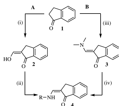
Scheme 1. Reagents and conditions: (i) NaOCH 3 /NaCH 3 /Et 2 O/0 °C, then H 2 O; (ii) R-NH 2 / p -TSA/CH 2 Cl 2 /reflux/1 h; (iii) DMFA/100 °C/1 h; (iv) R-NH 2 / p -TSA/EtOH/reflux/4 h.
