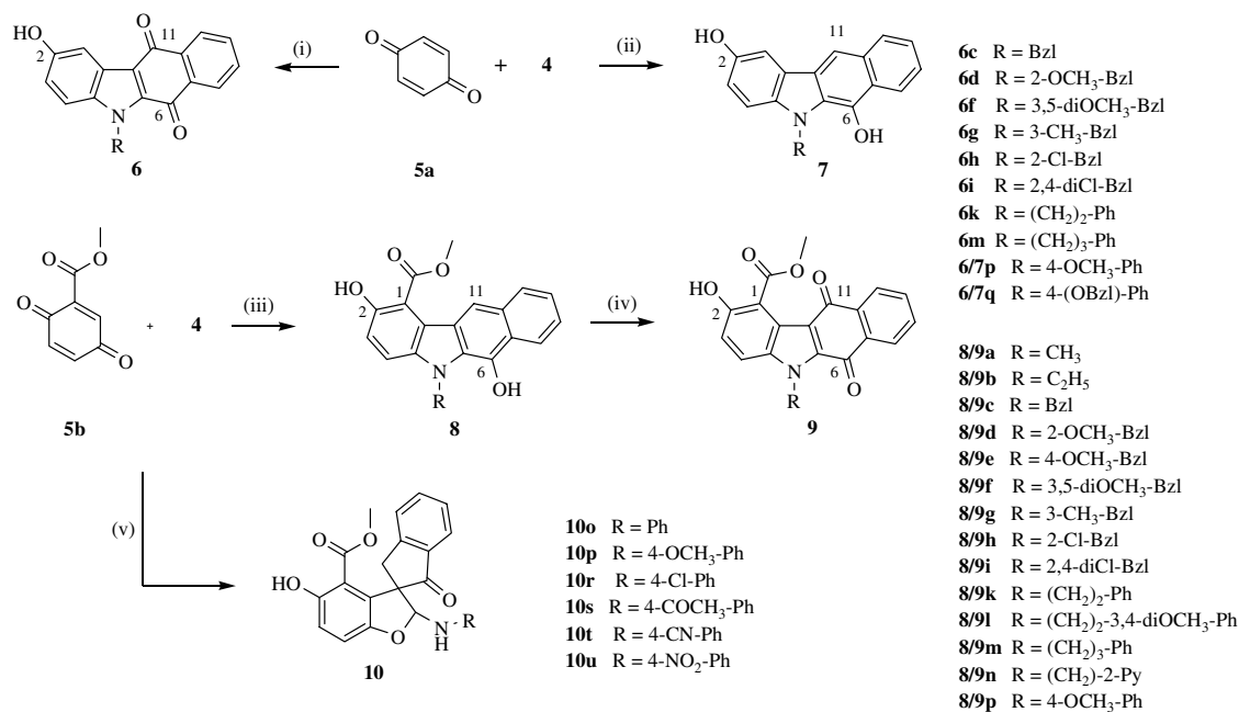
Scheme 2. Reagents and conditions: (i) 4equiv 4 /HOAc/rt/16h; (ii) 1equiv 4 /HOAc/argon/rt/30min; (iii) 1equiv 4 /HOAc/rt/15min; (iv) acetone/NaOH/rt/24h; (v) 1equiv 4 /HOAc/ \Delta T .
