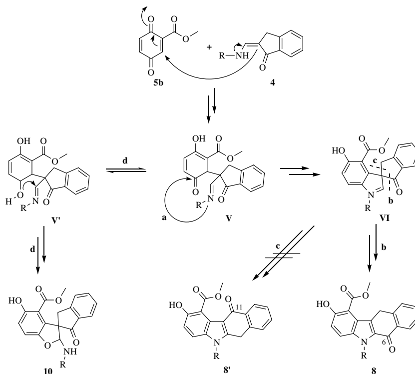
Scheme 3. Proposed mechanism for the formation of the 5H-benzo[b]carbazoles 8 and the spirocyclic benzofuran derivatives 10 .
