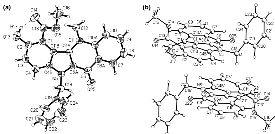
Figure 2. (a) Diagram of 15c . Displacement ellipsoids are drawn at the 50% probability level, radii of hydrogen atoms are chosen arbitrarily, and the hydrogen atom labels are omitted for clarity. Selected geometric features: C11–C12 1.322(3), C11–C11A 1.448(3), C11–C10A 1.475(3), C11A–C5A 1.379(2), C10A–C6A 1.386(3), C5A–C6 1.450(3), C6A–C6 1.470(3), C6–O25 1.223(2), C5A–N5 1.369(3), C4B–N5 1.368(2), C18–N5 1.472(3), C4B–C11B 1.395(2), C11B–C11A 1.433(3), O17–H17 0.94(2), H17···O14 1.69(3), O17···O14 2.578(3) Å; O15–C13–C1–C11B –19.7(3), C13–C1–C11B–C11A –22.6(4), C1–C11B–C11A–C11 –17.1(5), C11B–C11A–C11–C12 –15.0(4), C12–C11–C10A–C10 23.3(4), C4B–N5–C18–C19 –77.9(3)°. (b) View of the dimer of 15c formed in crystals, which is stabilized by \pi – \pi interactions (N5···C4B' 3.455 Å); atomic radii are chosen arbitrarily.
