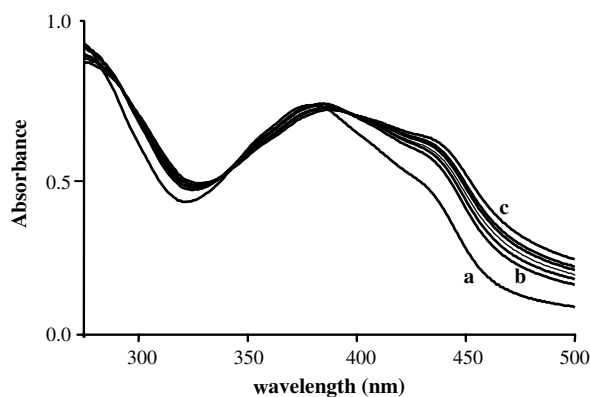
Figure 6. Time dependent UV spectra of 15c with calf thymus DNA. (a) 15c ( 5 \times 10^{-4} M) without DNA in Tris buffer (50 mM NaCl, 5 mM tromethamol), pH 7.2. (b) and (c) To 300 \mu L 15c were added 2200 \mu L Tris buffer and 500 \mu L of a concentrated DNA solution in Tris buffer: (b) incubation time: 5 min, (c) incubation time: 30 min.
